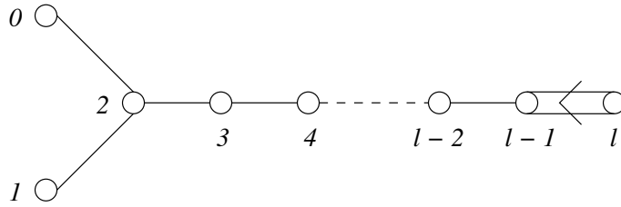
FIGURE 10. The Dynkin diagram of type A_{2l-1}^{(2)}
