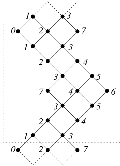
FIGURE 18. A full heap over the Dynkin diagram of type E_7^{(1)}
