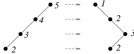
FIGURE 2. The heaps F and \overline{F} of Example 6.4
