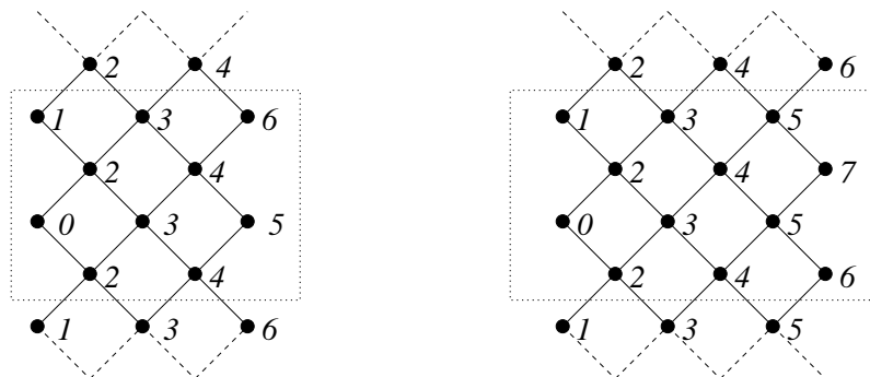
FIGURE 12. Full heaps over the Dynkin diagram of type D_l^{(1)} for l = 6 and l = 7
